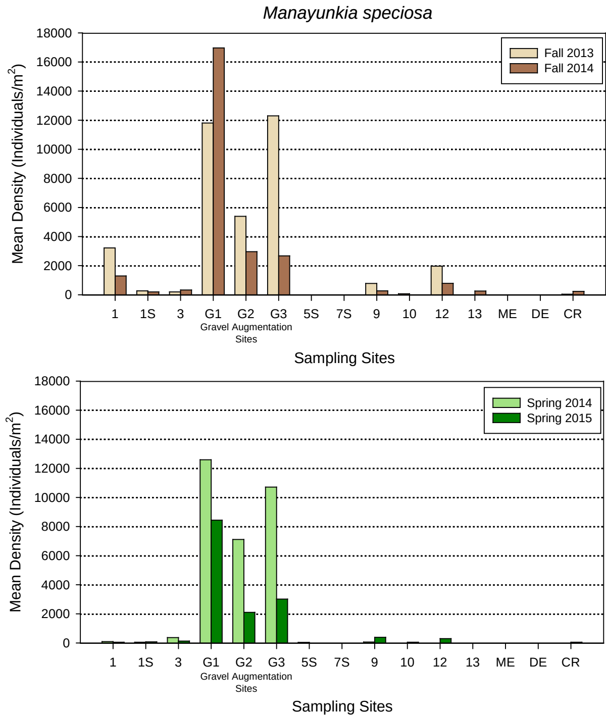
Figure 33. Density estimates of the polychaete Manayunkia speciosa in the lower Deschutes River downstream from the re-regulation dam and three reference sites.
