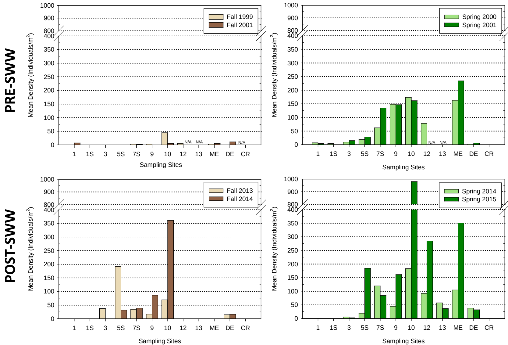
Appendix IV Figure 21. Epeorus spp. mayfly nymph densities in the lower Deschutes River downstream from the re-regulation dam and three reference sites for both baseline (Pre-SWW) and current (Post-SWW) studies.
