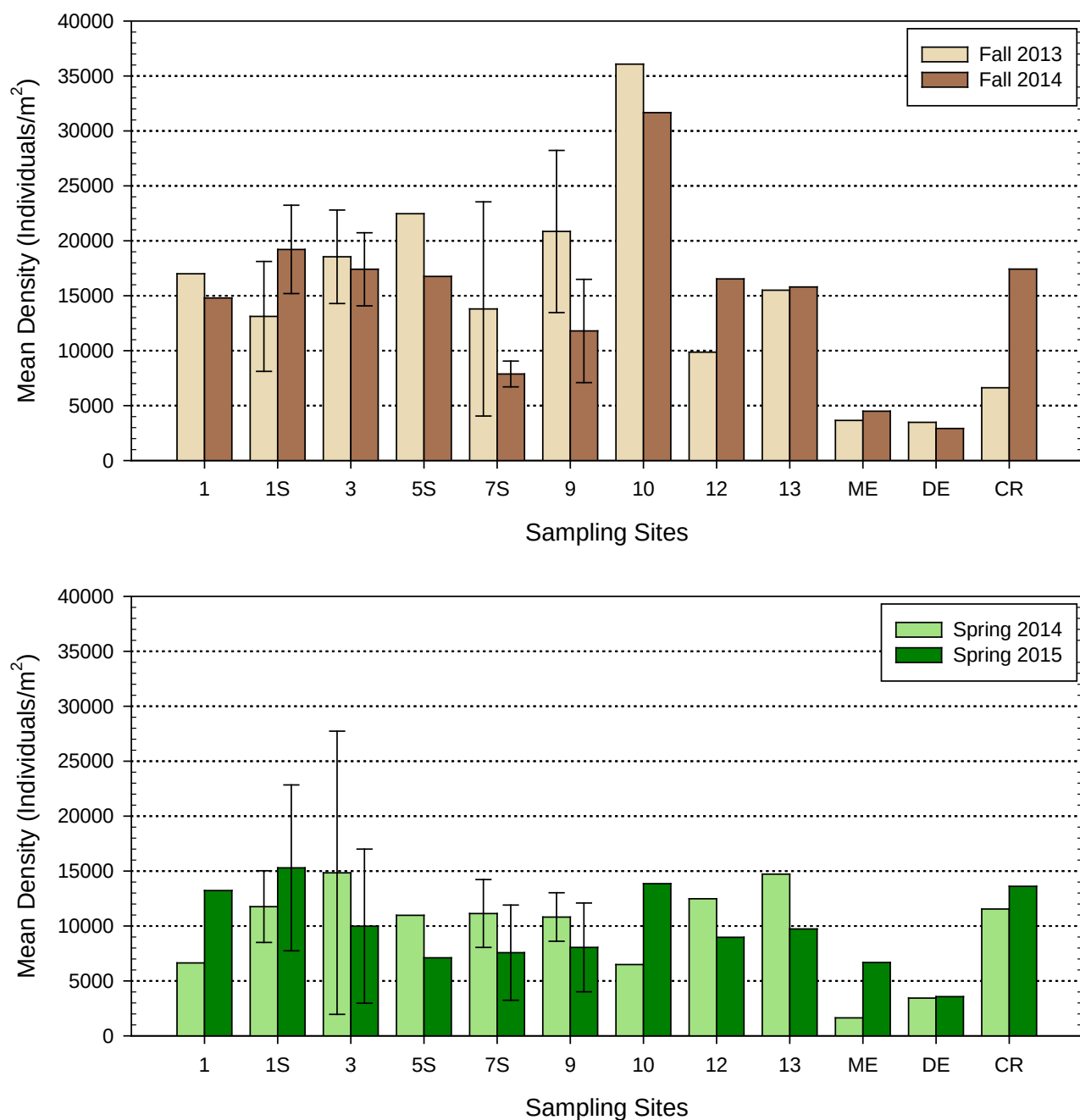
Appendix IV Figure 1. Mean benthic invertebrate densities in the lower Deschutes River downstream from the re-regulation dam and three reference sites for fall (upper) and spring (lower) collection efforts in 2013-2015. Those sites with replicate samples display 95% confidence intervals.
