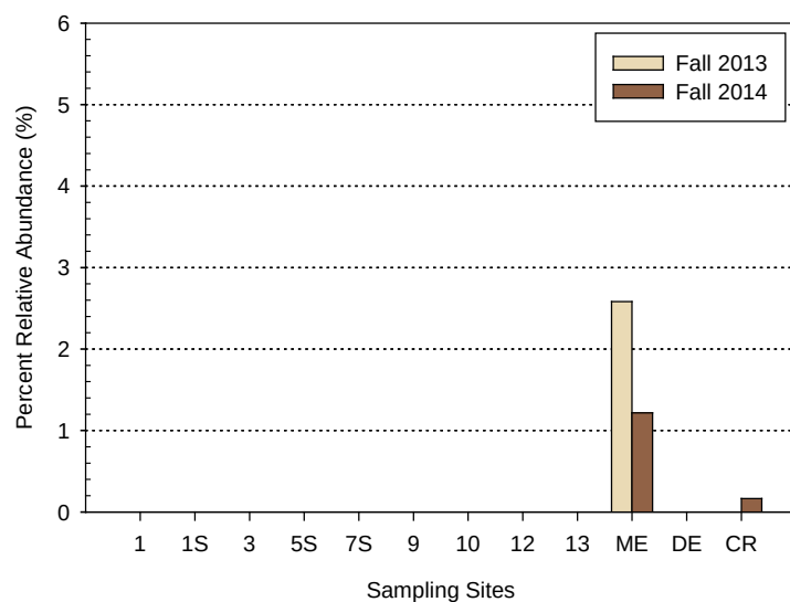
Figure 18. Antocha spp. cranefly larvae percent relative abundances in the lower Deschutes River downstream from the re-regulation dam and three upstream reference sites.
