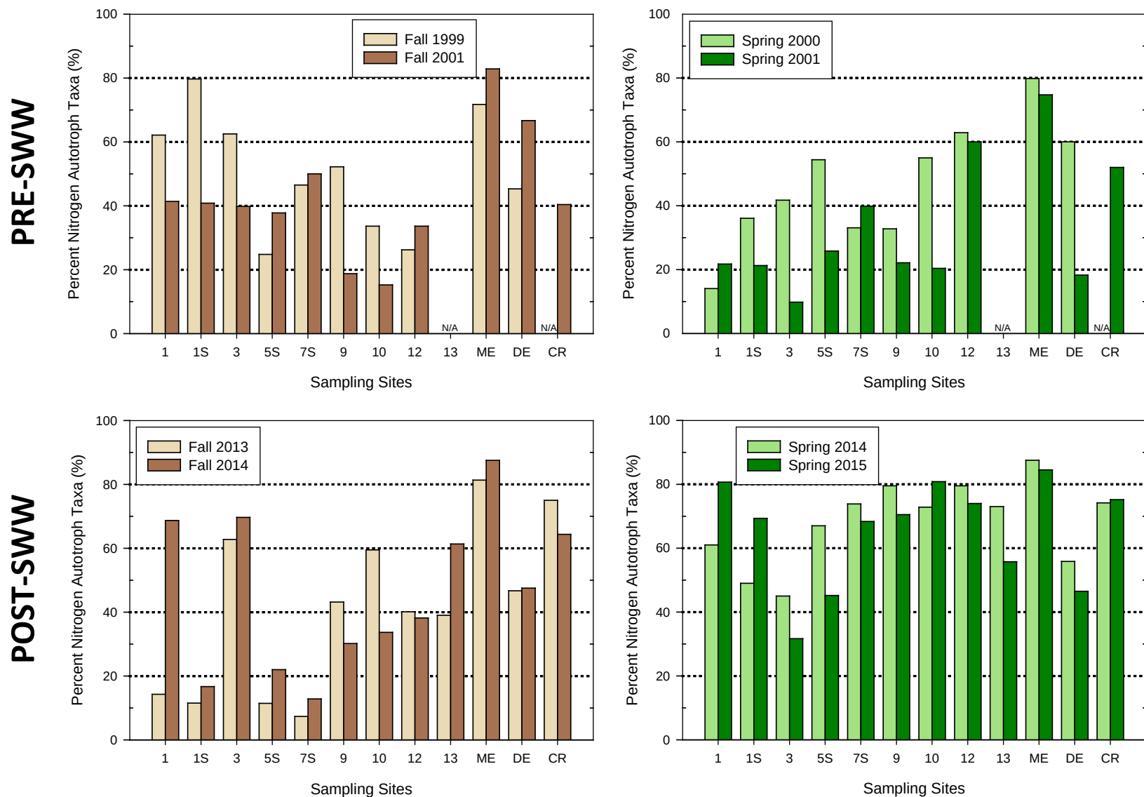
Appendix VII Figure 7. Percent relative abundances of diatom taxa classified as “nitrogen autotrophs” in composite periphyton samples collected from sites in the lower Deschutes River downstream from the re-regulation dam and three reference sites for both baseline (Pre-SWW) and current (Post-SWW) studies.
