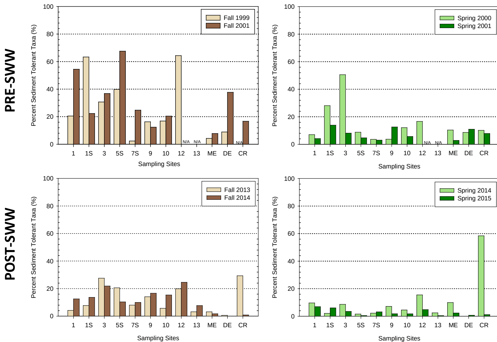
Appendix IV Figure 13. Relative abundances of benthic invertebrate taxa classified as “sediment tolerant” in the lower Deschutes River downstream from the re-regulation dam and three reference sites for both baseline (Pre-SWW) and current (Post-SWW) studies.
