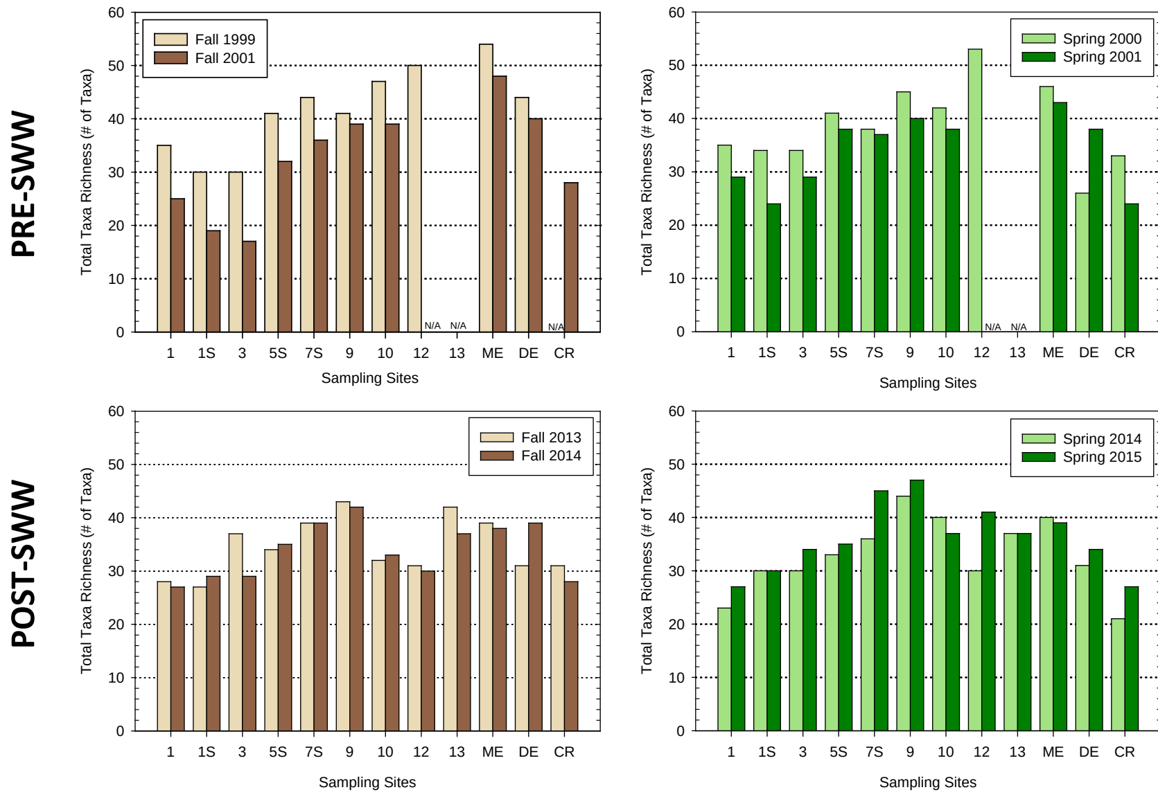
Figure 7. Benthic macroinvertebrate total taxa richness in the lower Deschutes River downstream from the re-regulation dam and three reference sites.
