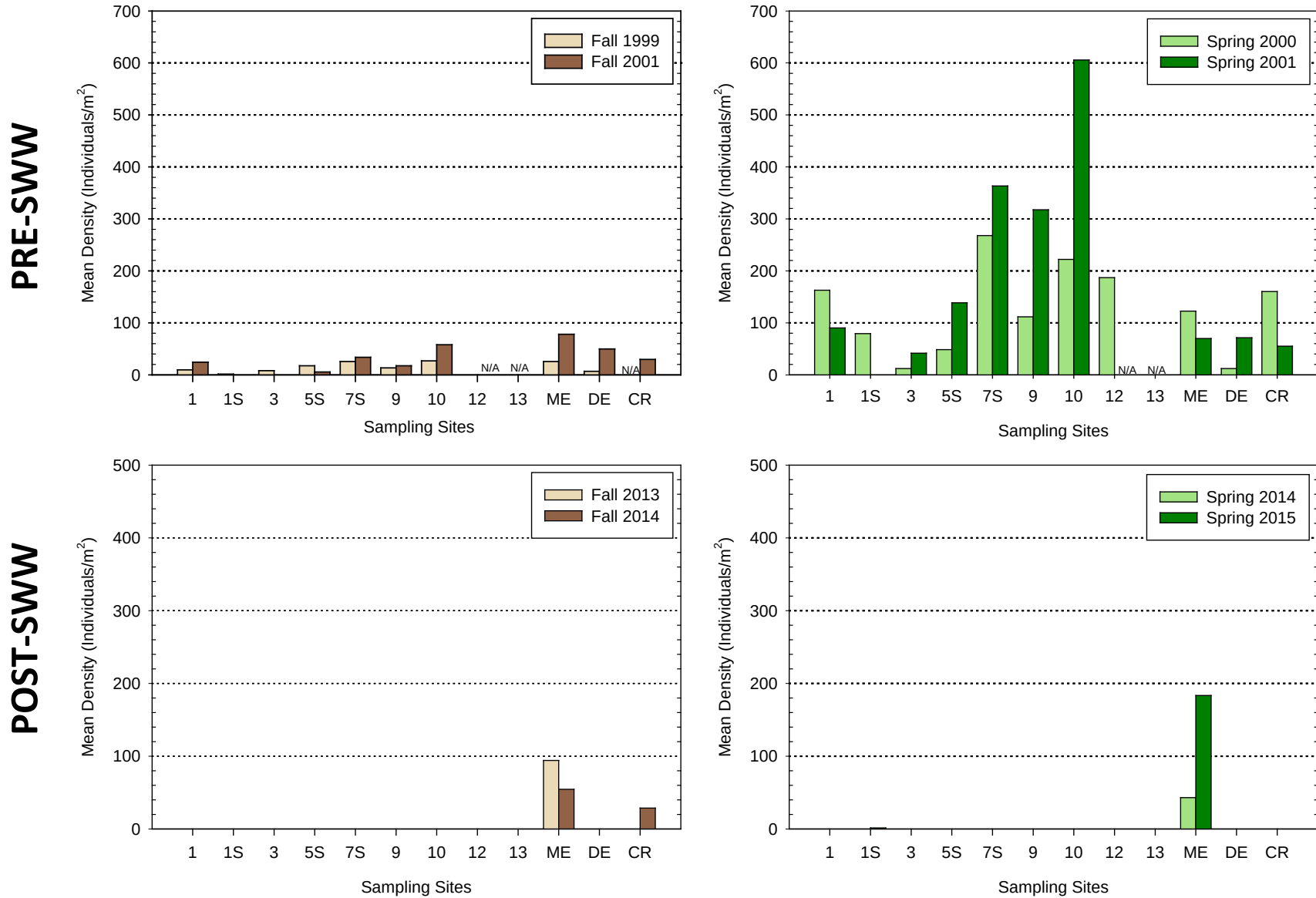
Figure 17. Antocha spp. cranefly larvae densities in the lower Deschutes River downstream from the re-regulation dam and at three upstream reference sites.
