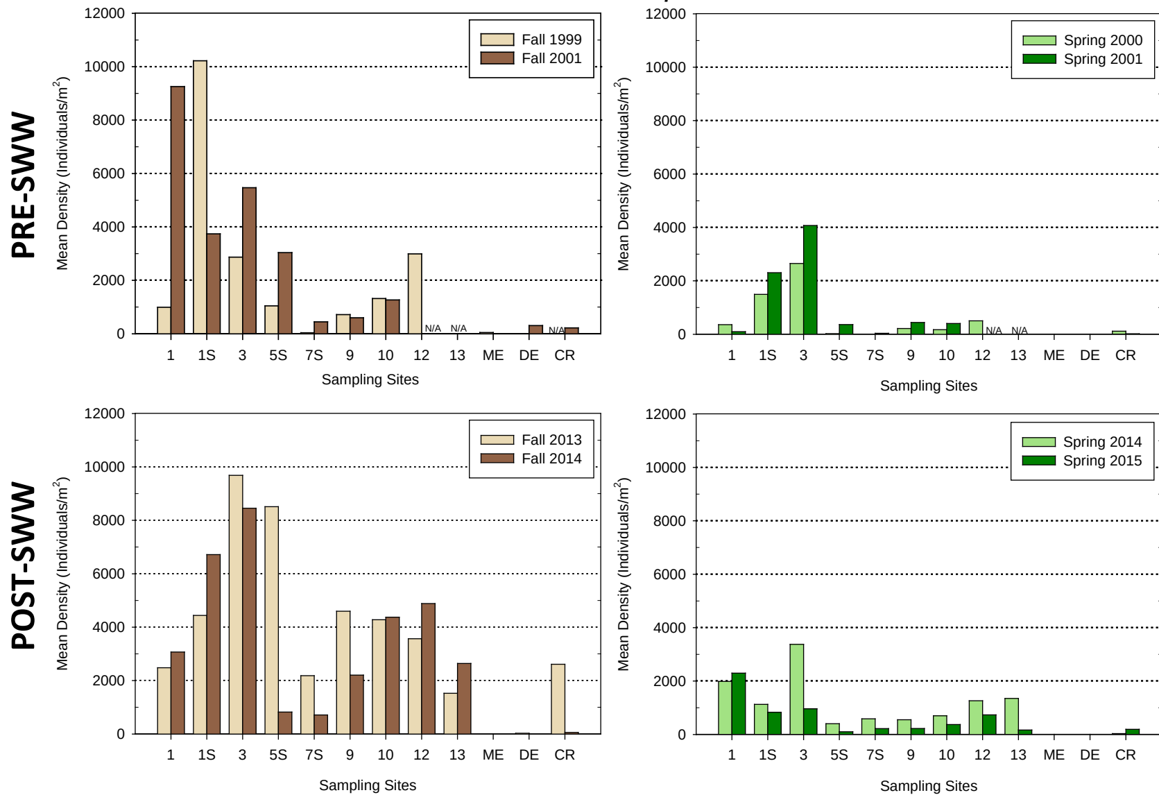
Figure 16. Gastropod (snails and limpets) densities in the lower Deschutes River downstream from the re-regulation dam and three upstream reference sites.
