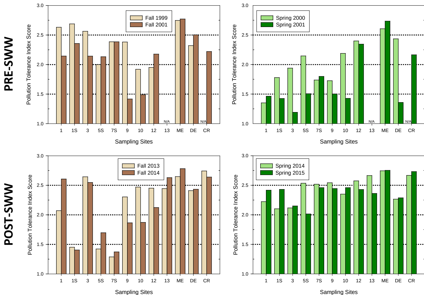
Appendix VII Figure 11. Pollution tolerance index (PTI) scores for diatom taxa in composite periphyton samples collected from sites in the lower Deschutes River downstream from the re-regulation dam and three reference sites for both baseline (Pre-SWW) and current (Post-SWW) studies. Scores range from 1 (most tolerant of pollution) to 3 (sensitive to pollution).
