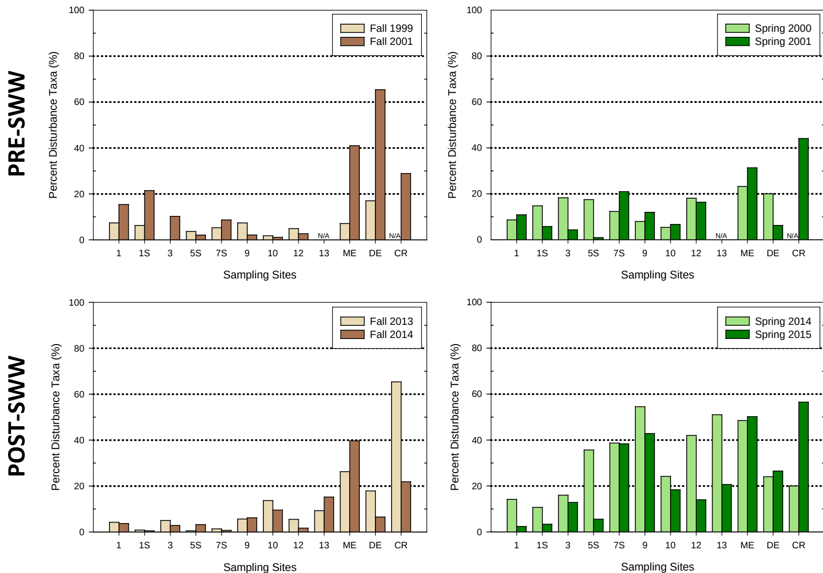
Appendix VII Figure 8. Percent relative abundances of diatom disturbance taxa Achnanthes minutissimum in composite periphyton samples collected from sites in the lower Deschutes River downstream from the re-regulation dam and three reference sites for both baseline (Pre-SWW) and current (Post-SWW) studies.
