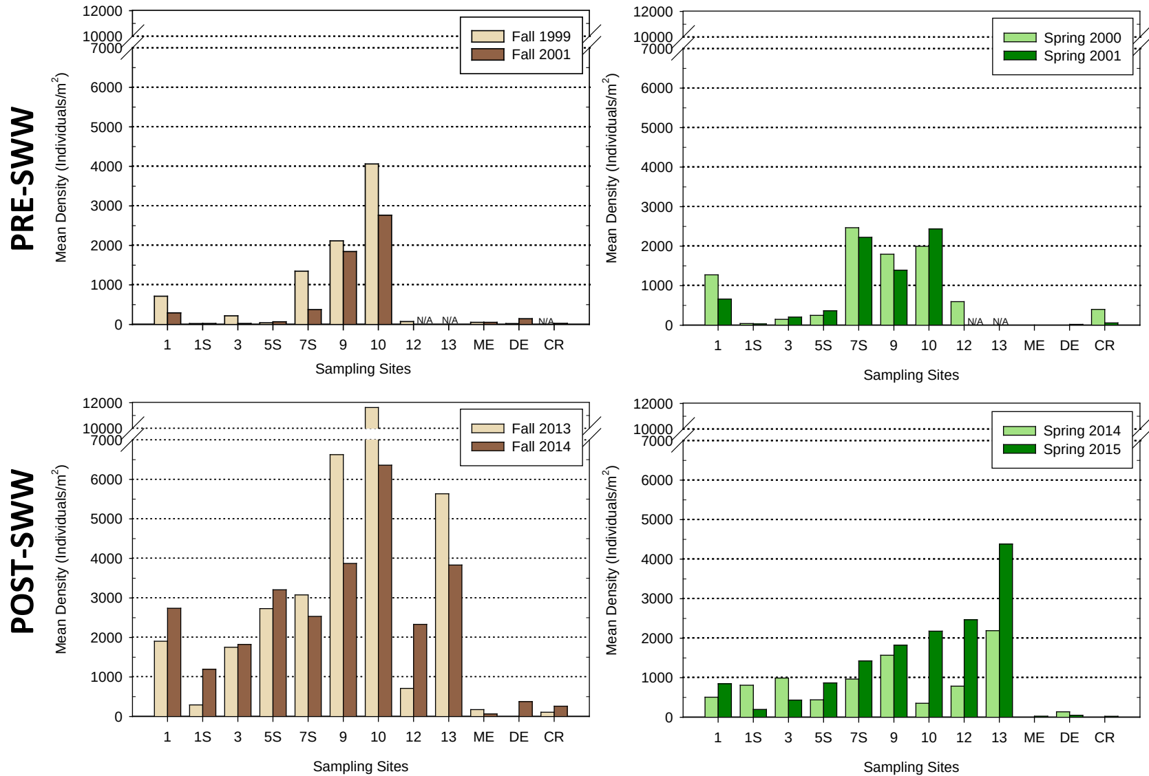
Appendix IV Figure 16. Hydropsychidae caddisfly larvae densities in the lower Deschutes River downstream from the re-regulation dam and three reference sites for both baseline (Pre-SWW) and current (Post-SWW) studies.
