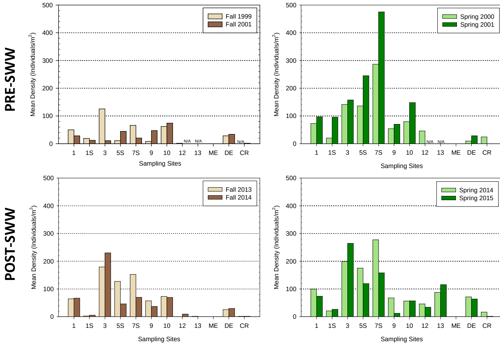
Appendix IV Figure 14. Pteronarcys stonefly nymph densities in the lower Deschutes River downstream from the re-regulation dam and three reference sites for both baseline (Pre-SWW) and current (Post-SWW) studies.
