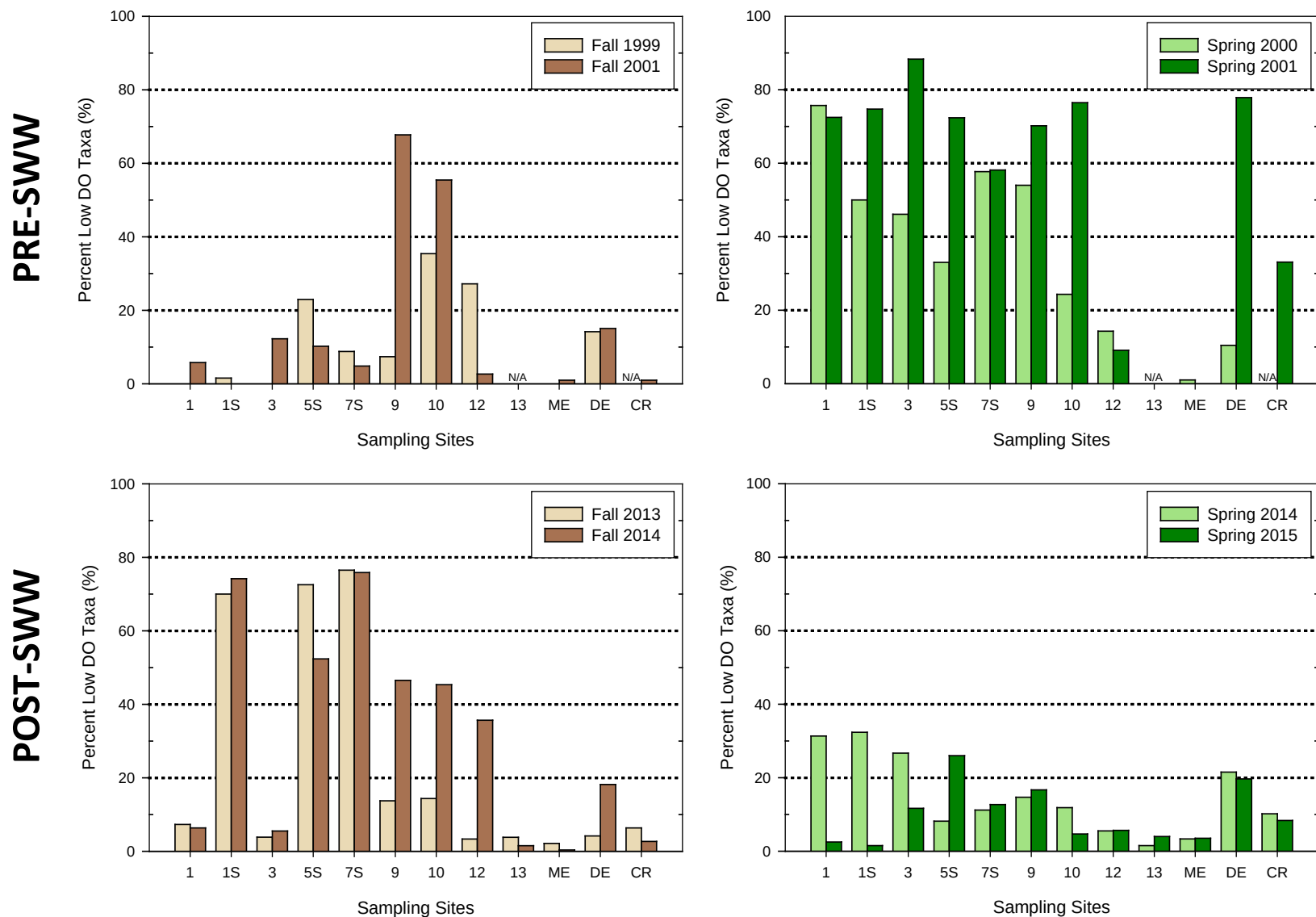
Appendix VII Figure 9. Percent relative abundance of low and very low oxygen demand diatom taxa in composite periphyton samples collected from sites in the lower Deschutes River downstream from the re-regulation dam and three reference sites for both baseline (Pre-SWW) and current (Post-SWW) studies.
